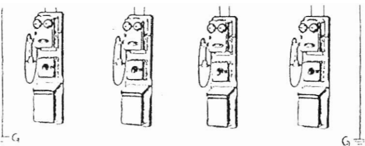
SERIES GROUNDING LINE
